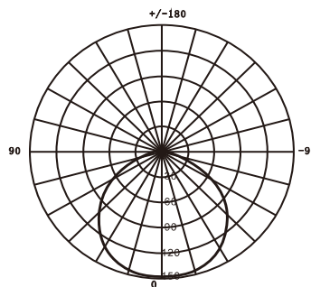
9W light distribution
